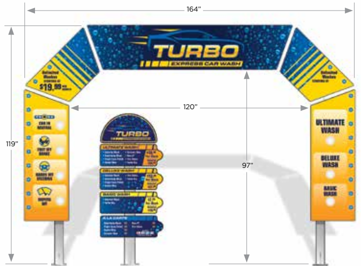
5 Piece Grand Arch Shown with Matching Sectional Menu
